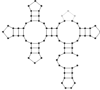
Figure 2.1: Example of a pseudoknot-free structure
