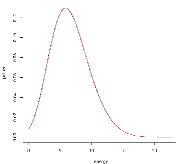
Figure 21: General EVD fits for the Salmonella (NC_003197) CyaR sRNA. (red: fit on unshuffled data, black: fit on shuffled data)
